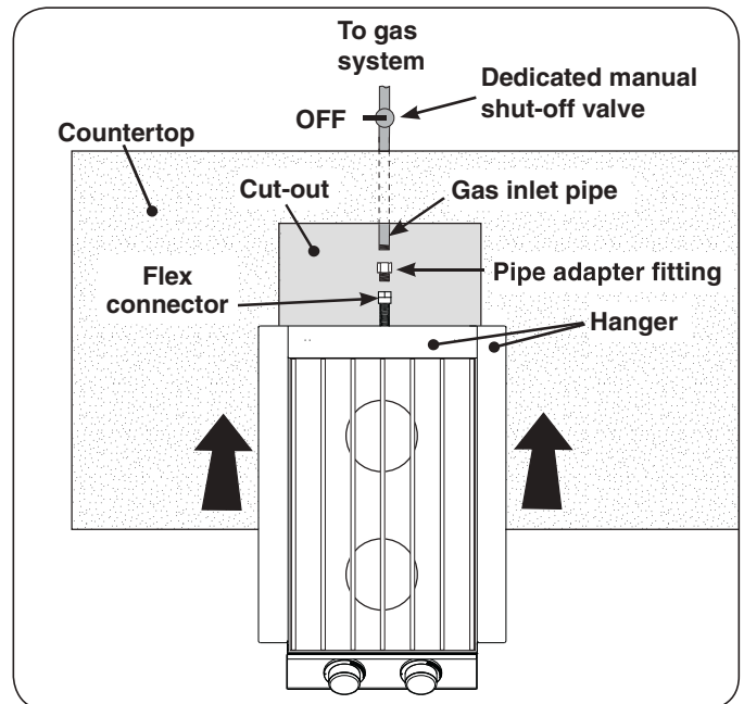
Fig. 11-3 Gas connection diagram
