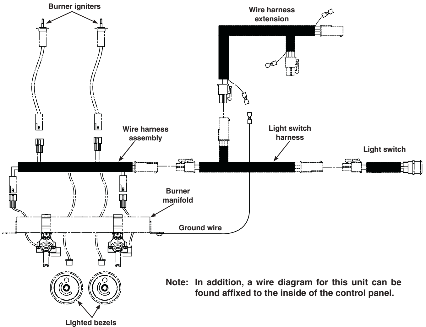
DOUBLE SIDEBURNER WIRING DIAGRAM
