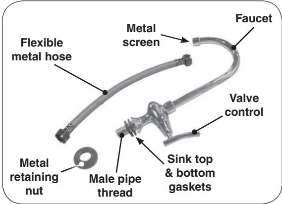
Fig. 1-1 Faucet detail
