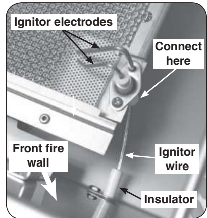
Fig. 4-1 Connect wire to electrode assy.
