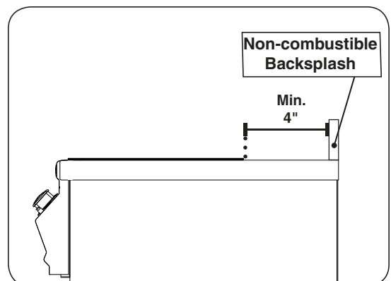
Fig. 8-4 Backsplash clearance
