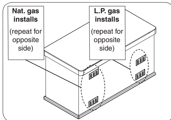
Fig. 10-1 Ventilation detail
