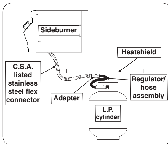
Fig. 10-2 Propane cylinder orientation
