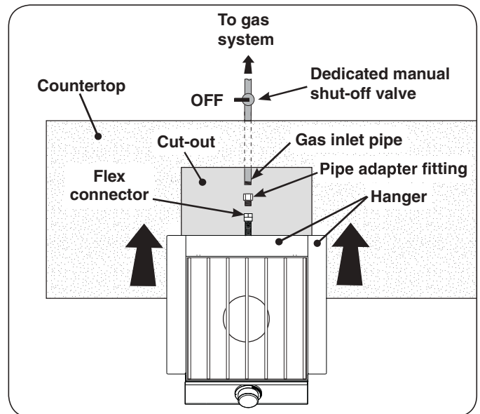
Fig. 11-3 Gas connection diagram
