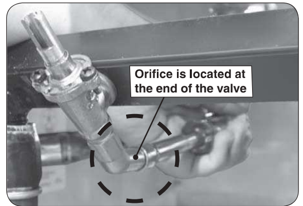
Fig. 13-2 Orifice location
